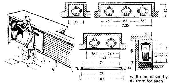
⑨ Space requirement for enclosed external waste bins
